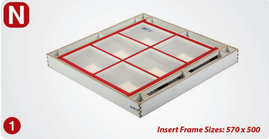
N Type Sieve Box With Wooden Insert Frame
